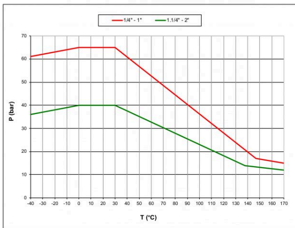
Pressure-temperature chart
